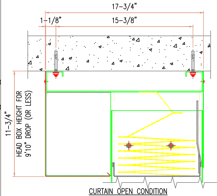
HEADBOX DETAIL
