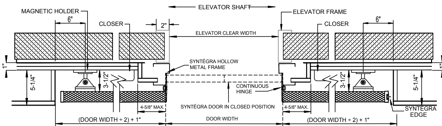
HORIZONTAL SECTION 2 NOT TO SCALE
